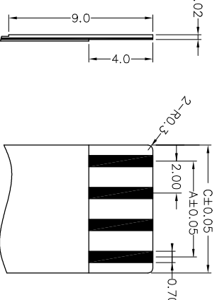
PROPER CABLE (SCALE 2:1)
