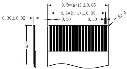
PROPER CABLE (SCALE 2:1)
